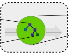
Commits
