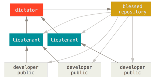
repositories
