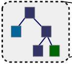
Trees
