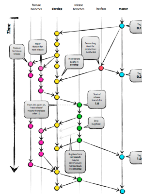
branches
