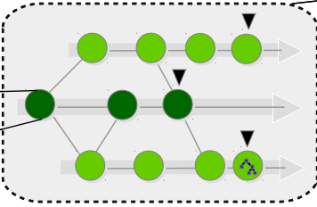
Branches
