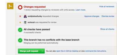
reviews
