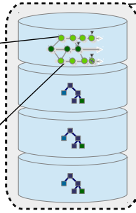
Repositories
